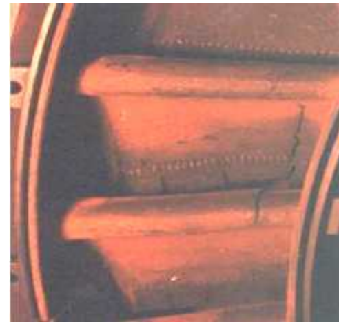
Turbine Nozzles at SCPS
